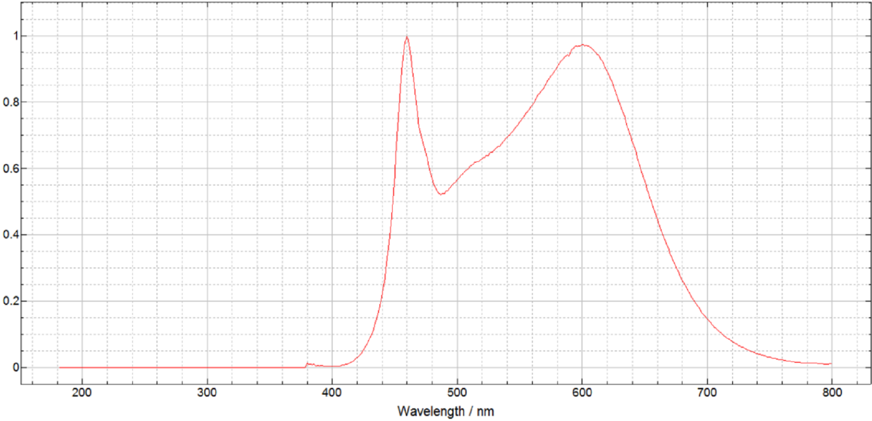
Appendix III: Spectral Power Distribution (Sample 1#)-Relative
